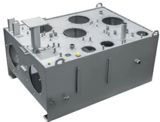
Special tank 1.400 L 1.4301, glass bead blasted
